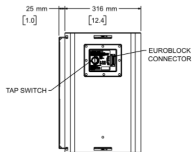
Rear View BRACKET SHOWN IN SIDE LOCATION
